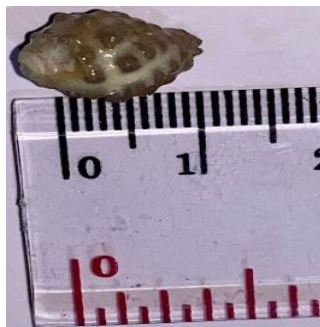
Species: Morula striata
