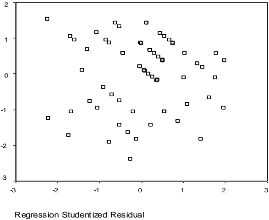
Scatterplot
