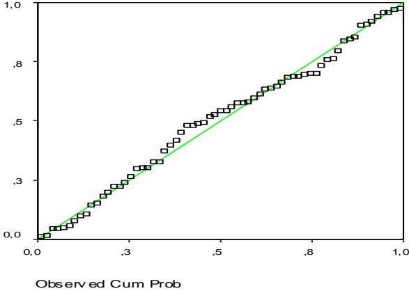
Scatterplot
